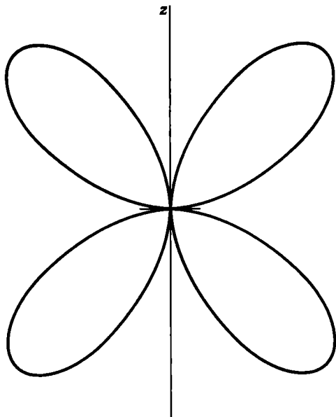
Figure 9.2 A quadrupole radiation pattern.
