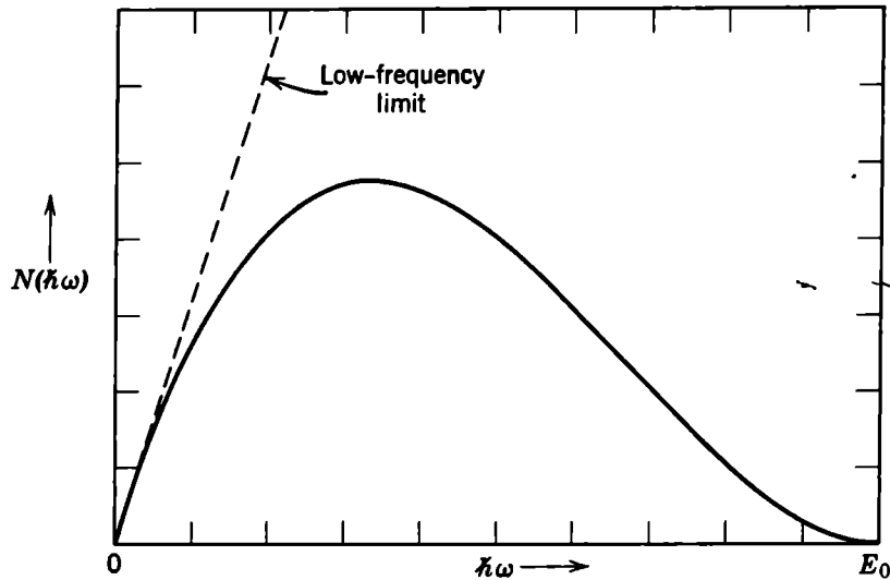
Figure 15.12 Spectrum of photons emitted in orbital-electron capture because of disappearance of the magnetic moment of the electron.
