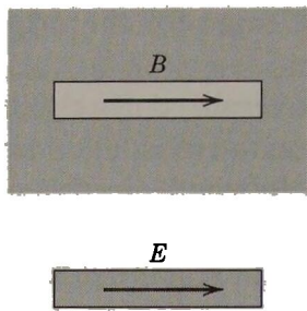
Figure 10.11 Equivalent radiators according to Babinet's principle.
