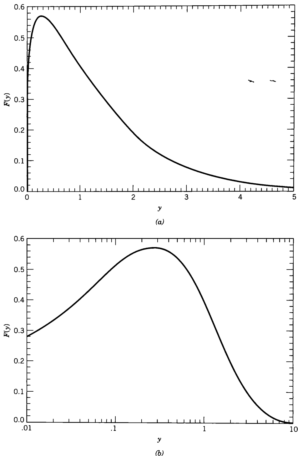
Figure 14.11 Normalized synchrotron radiation spectrum (1/I)(dI/dy) = (9\sqrt{3}/8\pi)y \int_y^\infty K_{5/3}(x) dx , where y = \omega/\omega_c and I = 4\pi e^2 \gamma^4/3\rho : (a) linear abscissa scale and (b) logarithmic abscissa scale.
