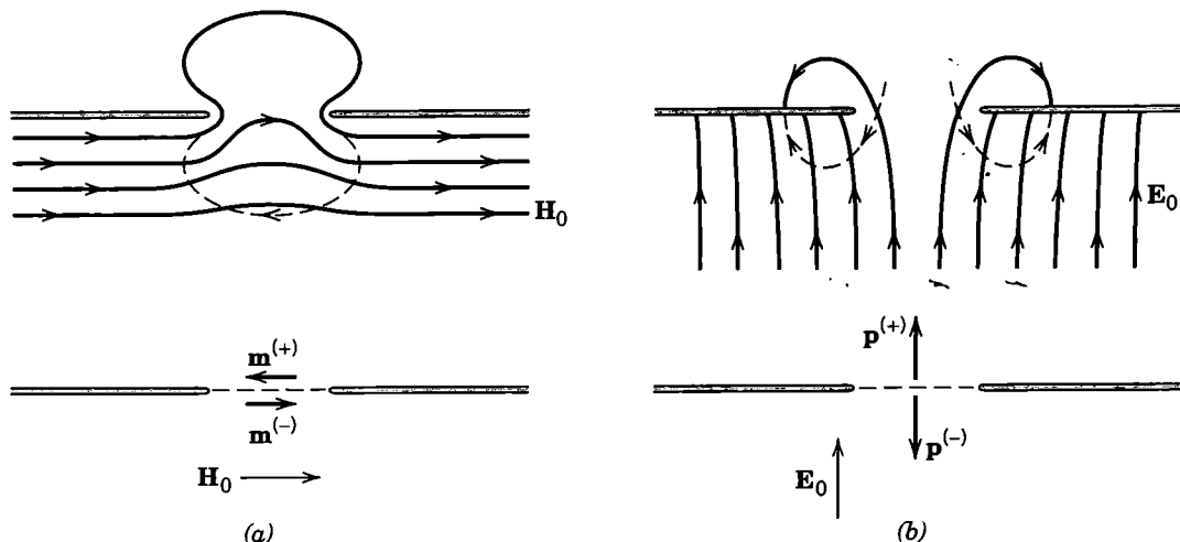
Figure 9.4 Distortion of (a) the tangential magnetic field and (b) the normal electric field by a small aperture in a perfectly conducting surface. The effective dipole moments, as viewed from above and below the surface, are indicated beneath.
