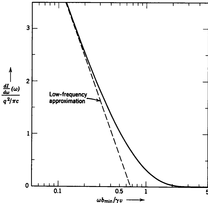
Figure 15.8 Frequency spectrum of virtual quanta for a relativistic particle, with the energy per unit frequency dI(\omega)/d\omega in units of q^2/\pi c and the frequency in units of \gamma v/b_{\min} . The number of virtual quanta per unit energy interval is obtained by dividing by \hbar^2\omega .
