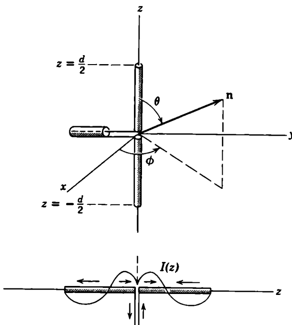
Figure 9.6 Linear, center-fed antenna.
