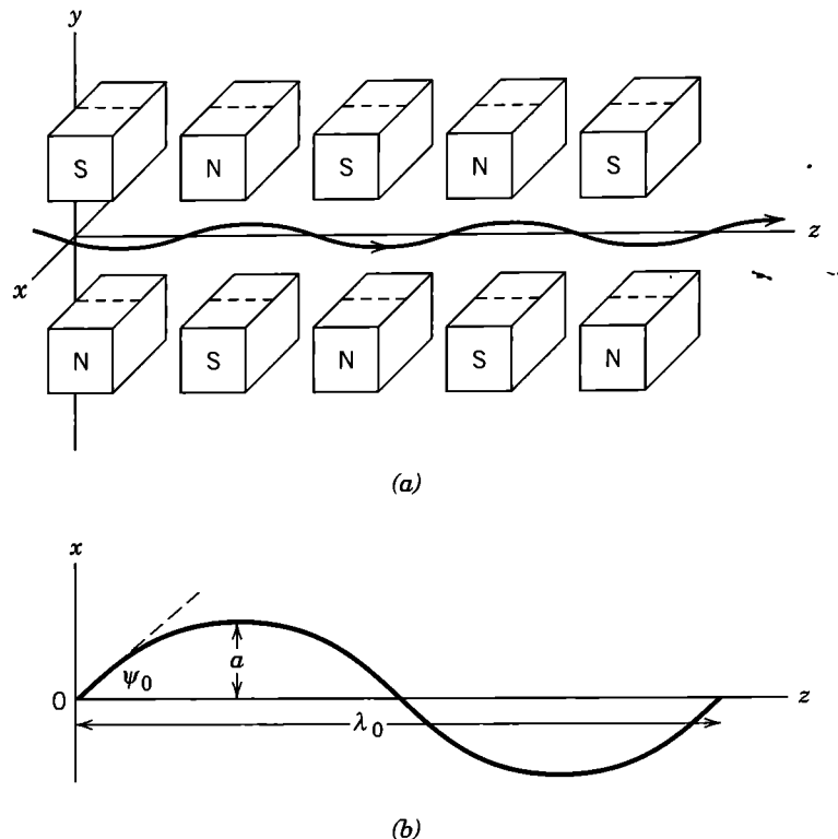
Figure 14.12 (a) Schematic diagram of alternating-polarity bending magnets for a wiggler or undulator. (b) Sketch of approximately sinusoidal path of electron in the x - z plane. The magnet period is \lambda_0 , the maximum transverse amplitude is a , and the maximum angle is \psi_0 .
