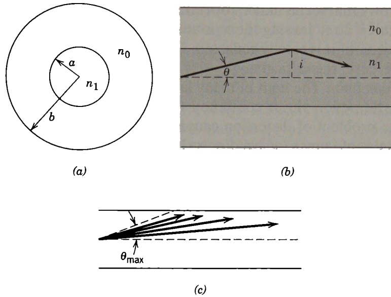
Figure 8.10 Optical fiber core and cladding, with inner cylinder of index of refraction n_1 and cladding of index n_0 ( n_1 > n_0 ): (a) cross section of fiber; (b) longitudinal section, showing a total internally reflected ray; (c) longitudinal section of the core, showing meridional propagating rays with complementary angles of incidence \theta < \theta_{\max} = \cos^{-1}(n_0/n_1) , the critical angle for total internal reflection.
