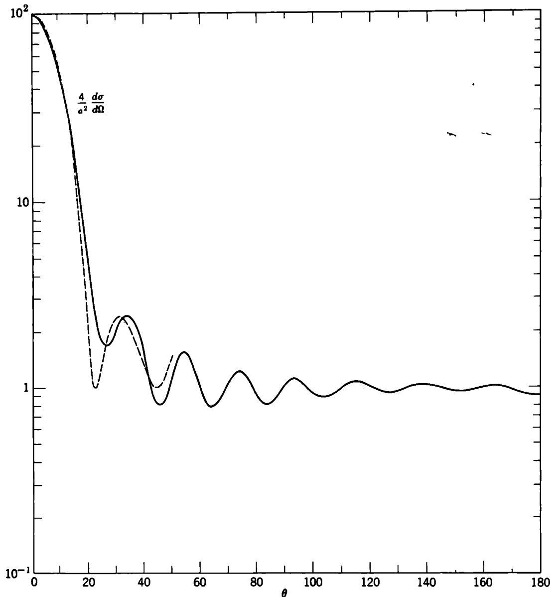
Figure 10.16 Semilogarithmic plot of the scattering cross section for a perfectly conducting sphere as a function of scattering angle, with an unpolarized plane wave incident and ka = 10 . The solid curve is the exact result ( King and Wu ). The dashed curve is the approximation based on the sum of the amplitudes (10.127) and (10.132).
