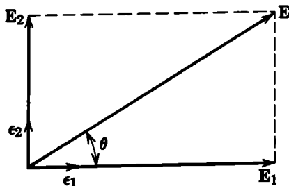
Figure 7.2 Electric field of a linearly polarized wave.
