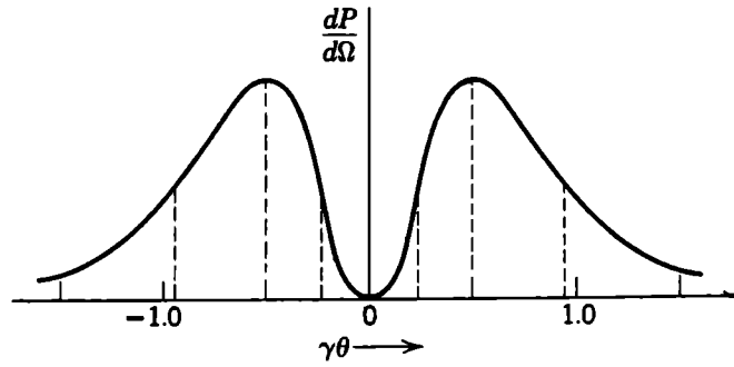
Figure 14.5 Angular distribution of radiation for relativistic particle.
