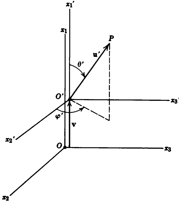
Figure 11.4 Addition of velocities.
