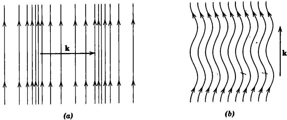
Figure 7.12 Magnetohydrodynamic waves.
