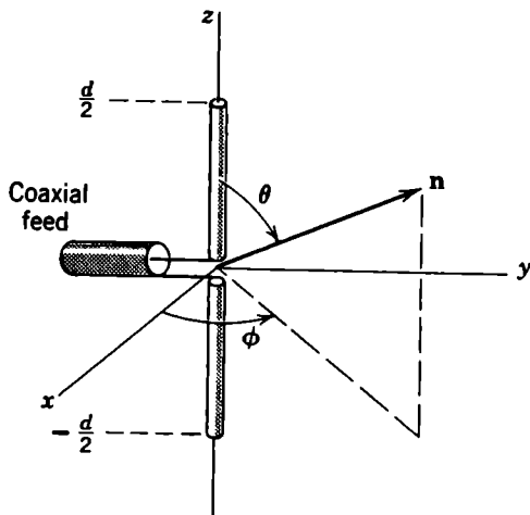
Figure 9.3 Center-fed, linear antenna.
