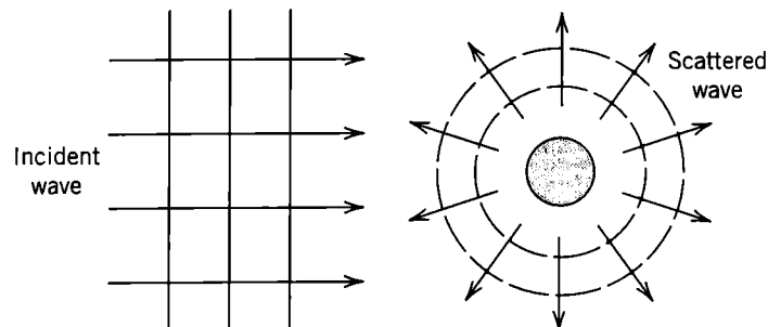
Figure 10.6 Scattering of radiation by a localized object.
