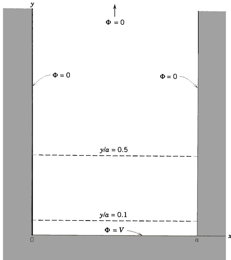
Figure 2.10 Two-dimensional potential problem.
