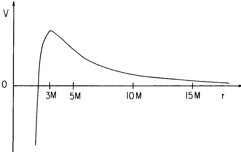
Fig. 6.5. The effective potential, V , for null geodesics.
