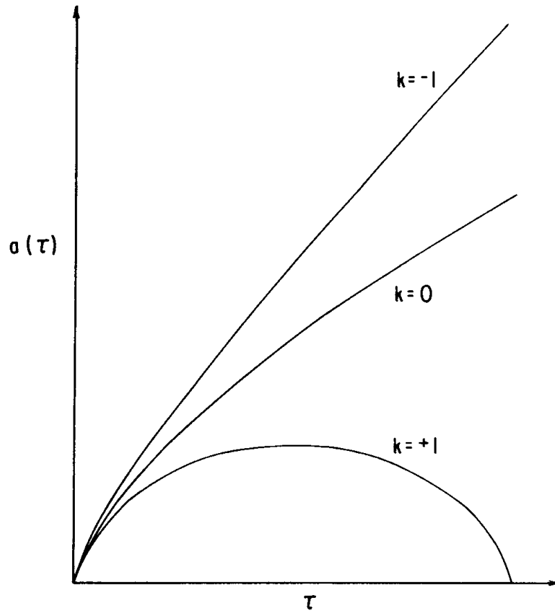
Fig. 5.4. The dynamics of radiation-filled Robertson-Walker universes.
