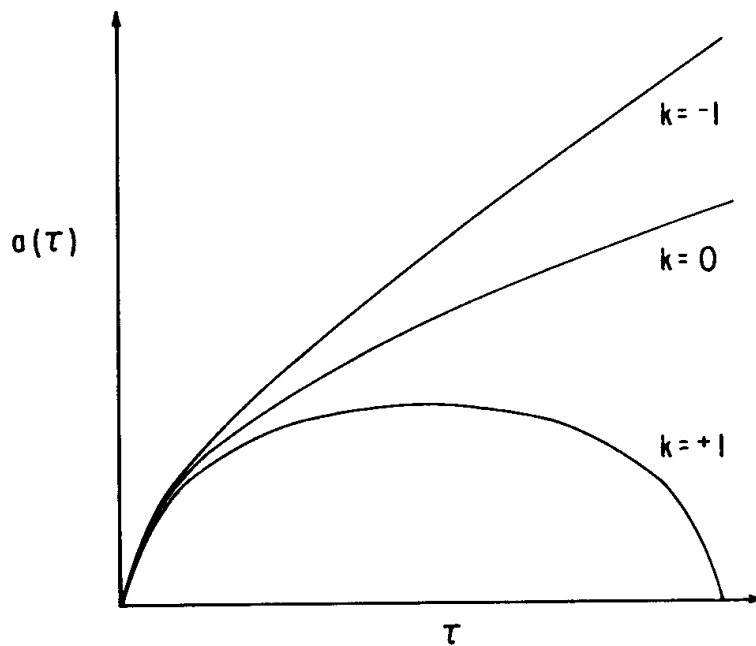
Fig. 5.3. The dynamics of dust-filled Robertson-Walker universes.
