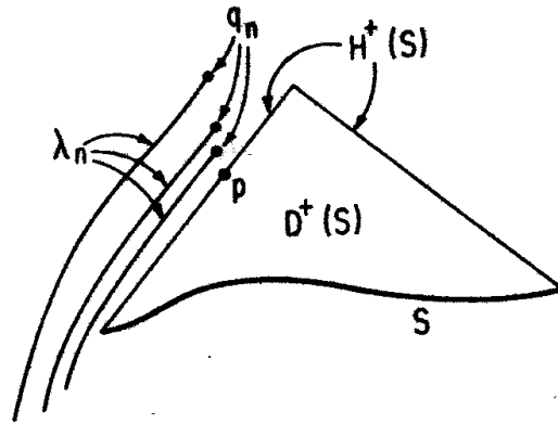
Fig. 8.13. A point p \in H^+(S) \cap I^+(S) with a sequence of points q_n \in I^+(p) converging to p (see theorem 8.3.5).
