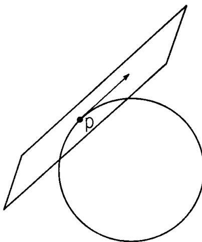
Fig. 2.2. The tangent plane at point p of a sphere in \mathbb{R}^3 .
