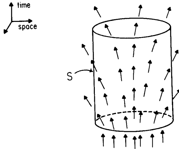
Fig. 4.1. A spacetime diagram showing the mass-energy current density J^a in a volume V of spacetime.
